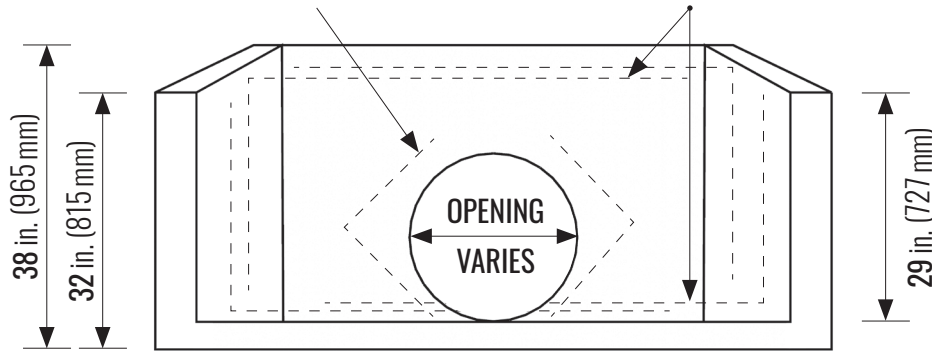
FRONT X-SECTION
