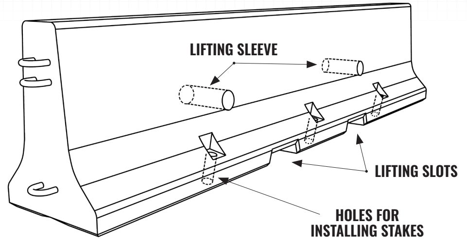
PERSPECTIVE VIEW
