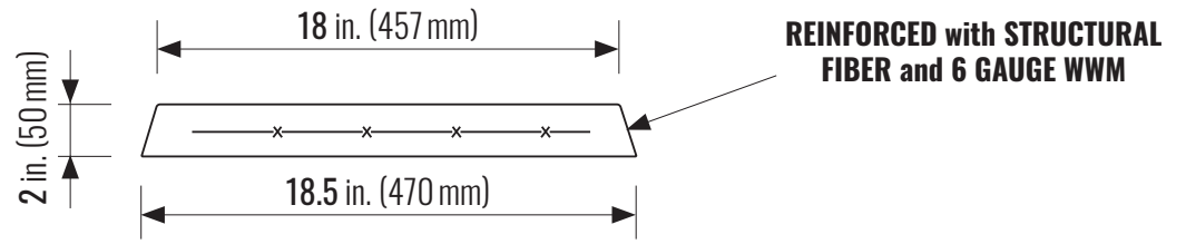
FRONT X-SECTION
