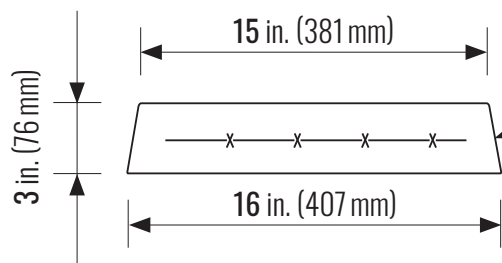
FRONT X-SECTION
