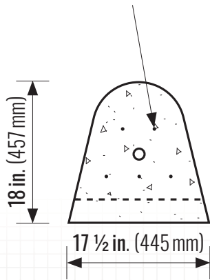
END X-SECTION
