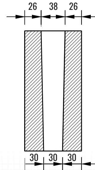
END X-SECTION
