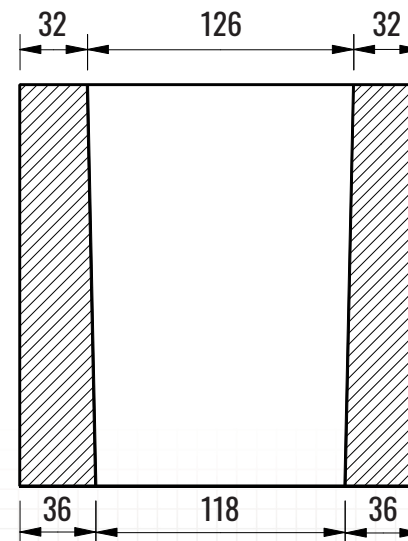
END X-SECTION
