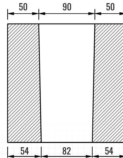
END X-SECTION
