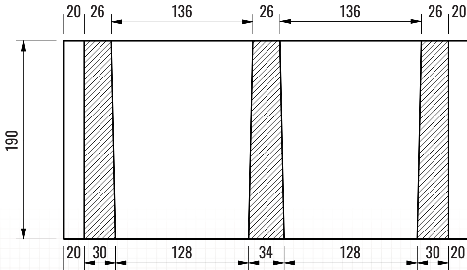
FRONT X-SECTION
