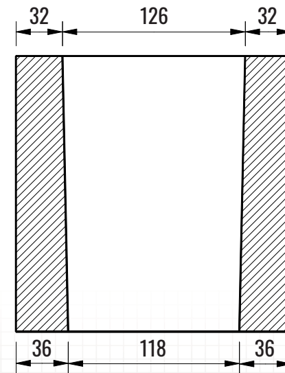
END X-SECTION
