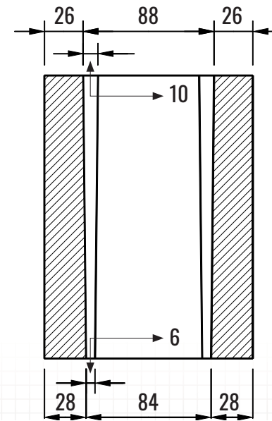
END X-SECTION
