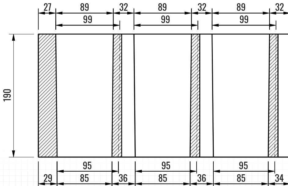
FRONT X-SECTION
