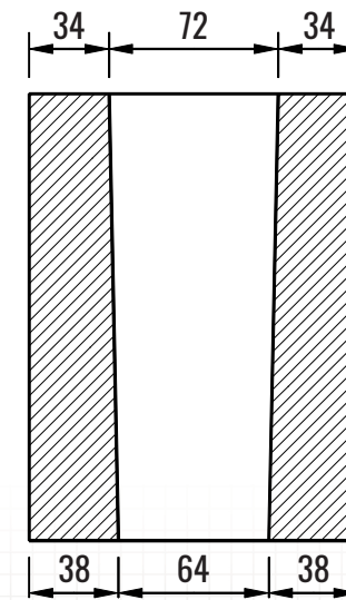
END X-SECTION
